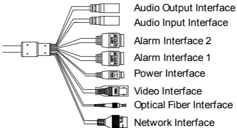
Figure 1-5 Cable Description
