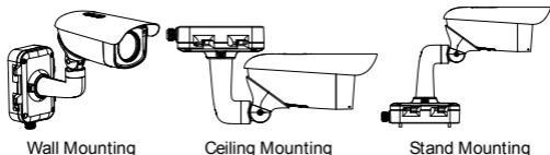
Figure 2-6 Type I Camera Installation Methods
